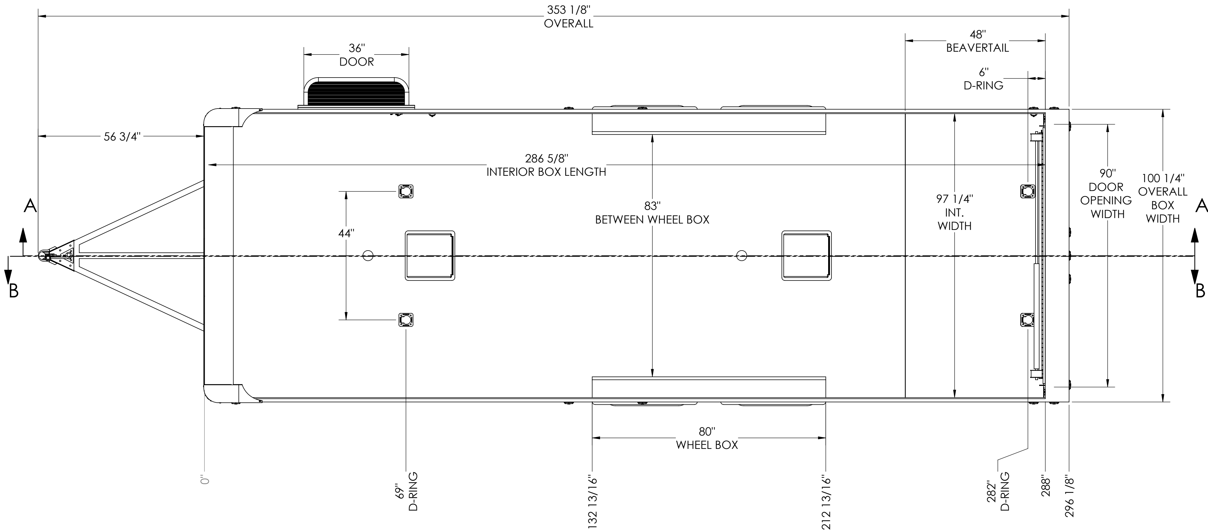
TOP VIEW STANDARD FLOOR LAYOUT
