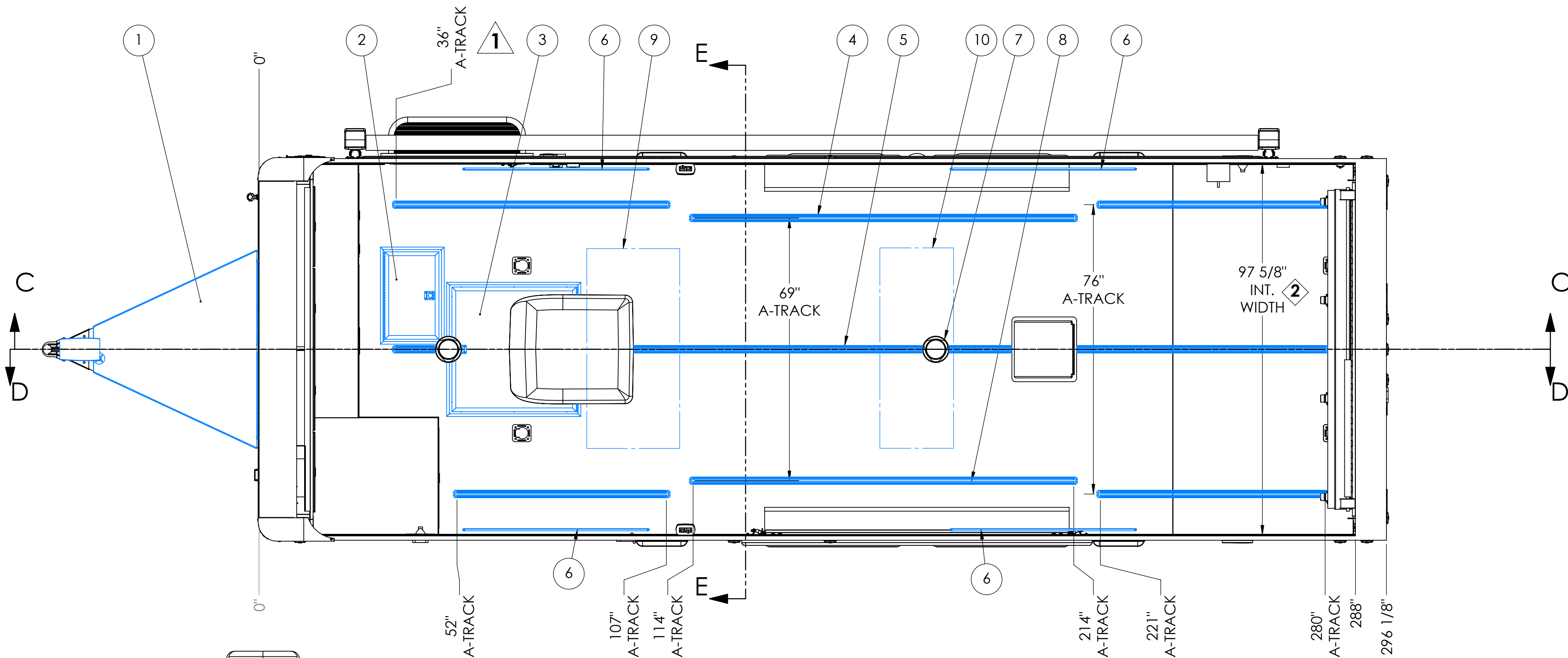
TOP VIEW POPULAR OPTIONS FLOOR LAYOUT
