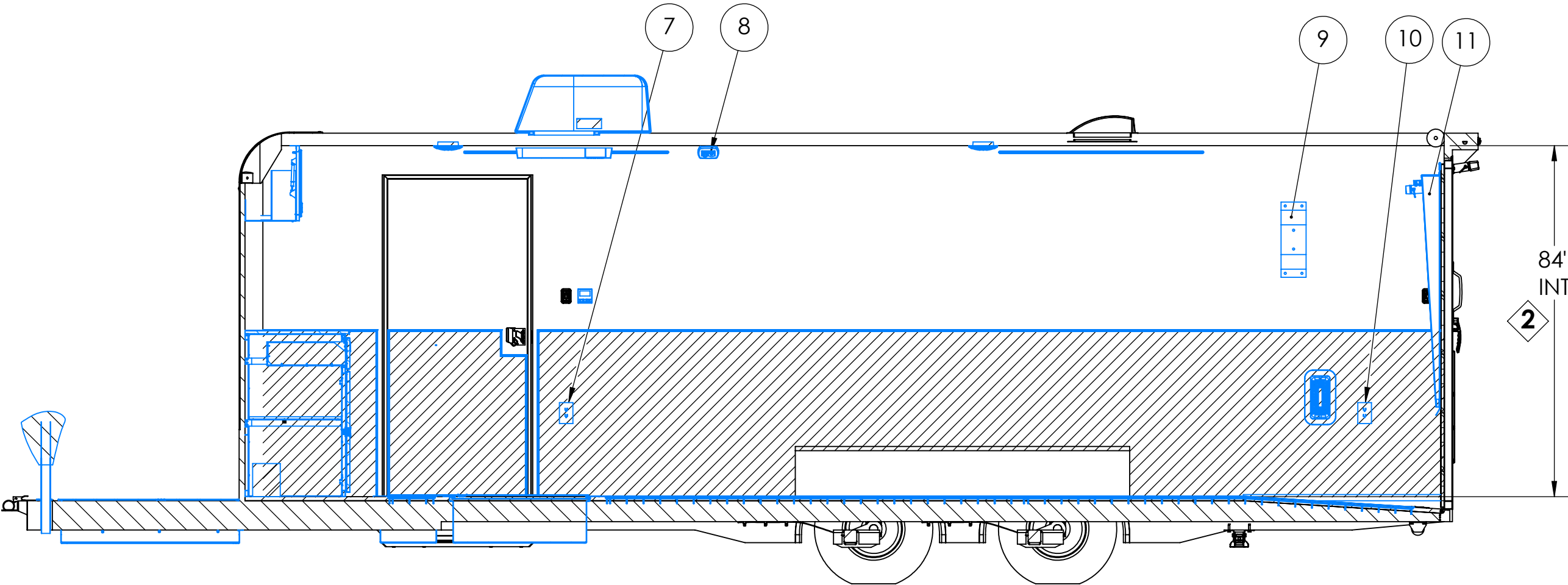
SECTION C-C SCALE 1 : 28
